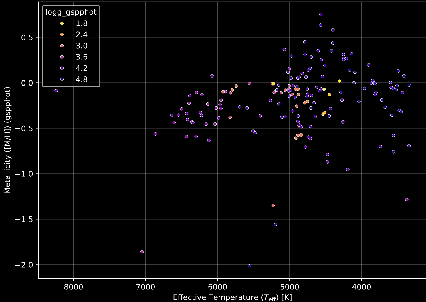
APOGEE DR17 Field: [140+60] Stellar Population Parameters (n= 169)
