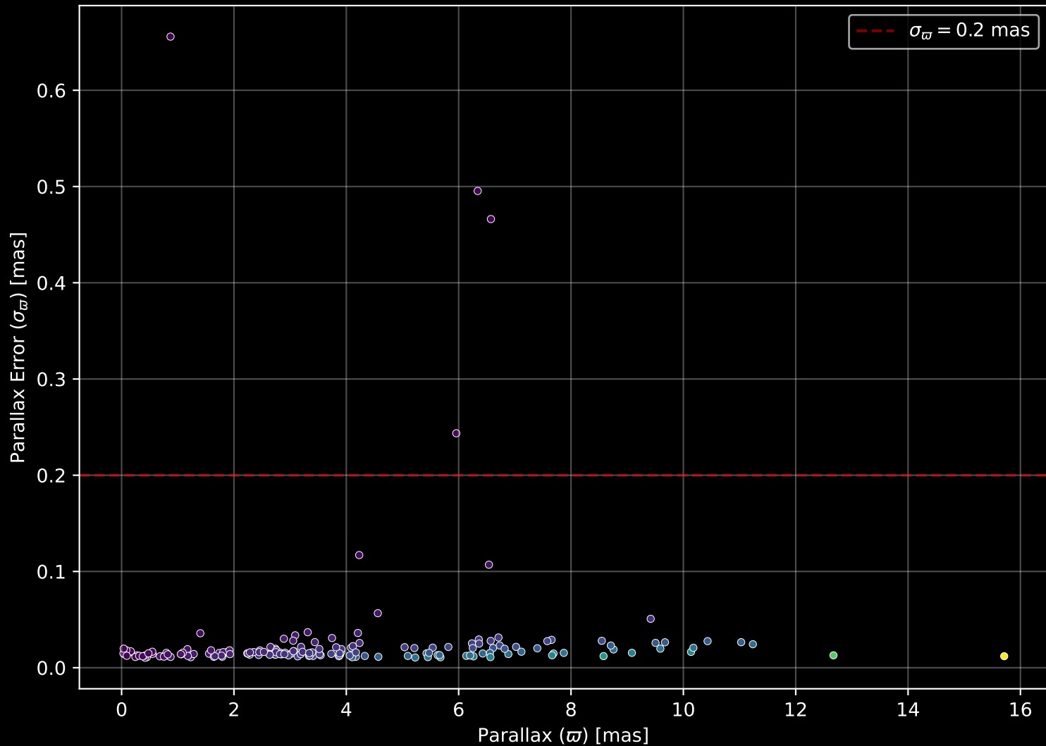
APOGEE DR17 Field: [140+60] Parallax Quality (n= 169)
