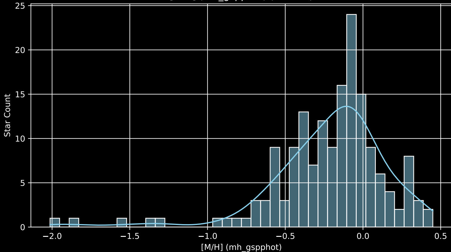
APOGEE DR17 Field: [140+60 [M/H] (mh_gspphot) (n= 166)
