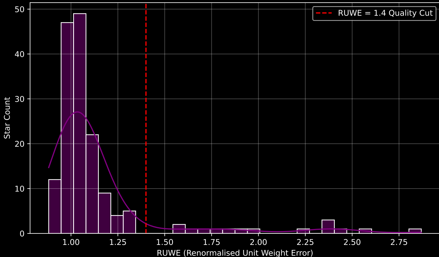
GAPOGEE DR17 Field [140+60] RUWE Distribution (n= 163)
