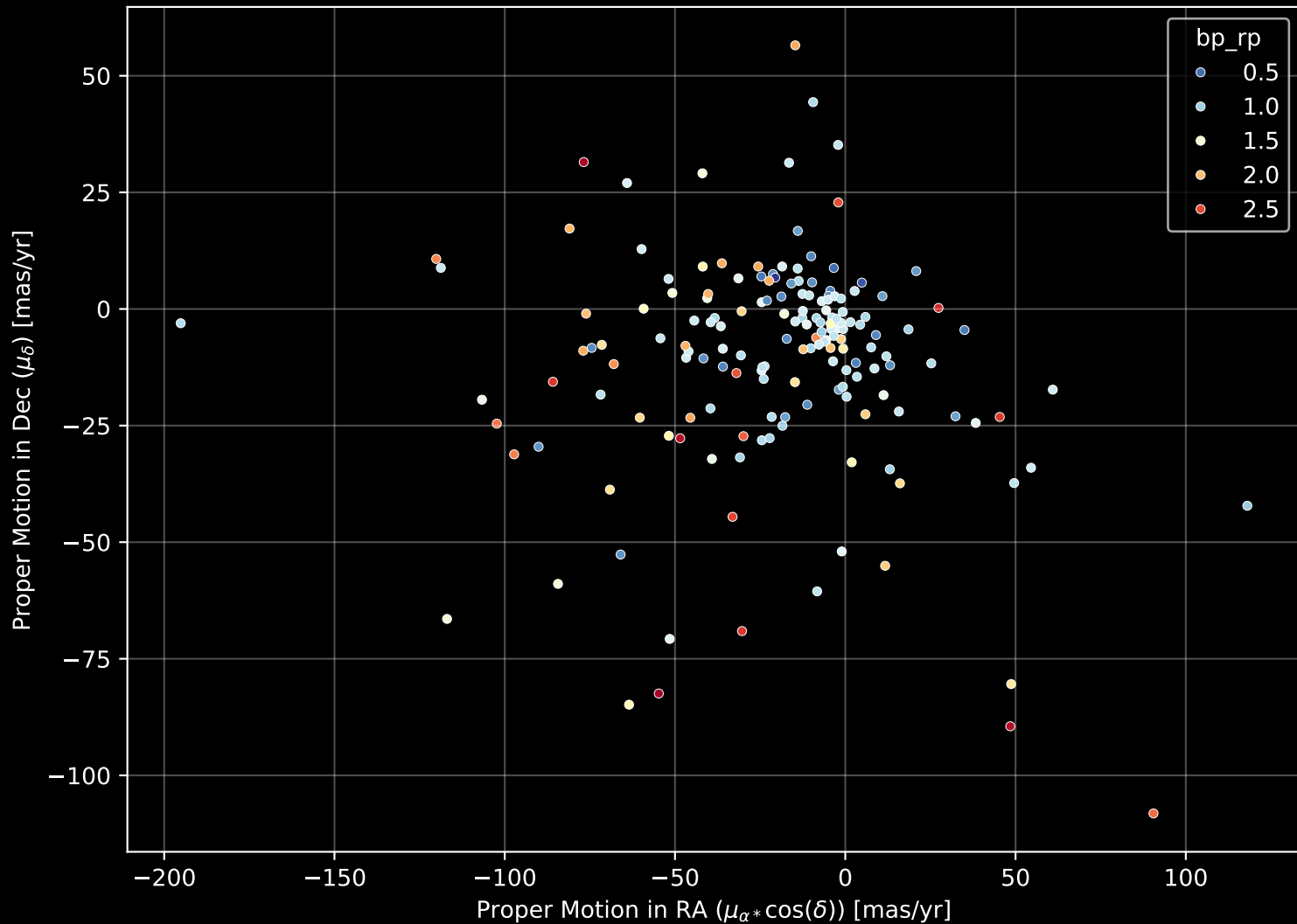
APOGEE DR17 Field: [140+60] Proper Motion Diagram (n= 169)
